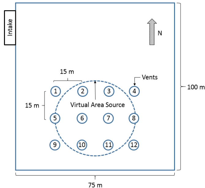
Figure 2.23. Multiple-vent release configuration for Example 5.
