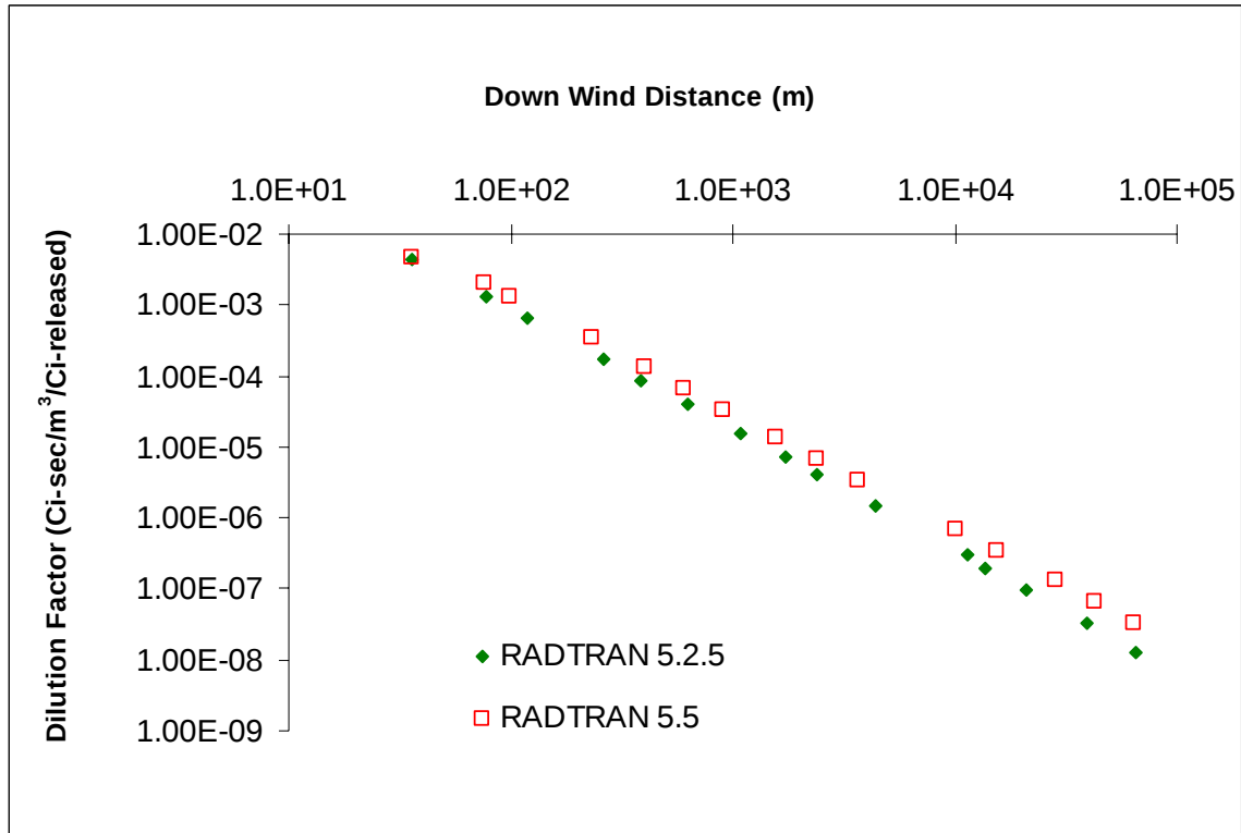
Figure 1: Atmospheric Comparison with RADTRAN 5 and RADTRAN 5.5
