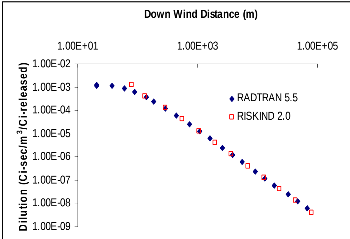
Figure 7: Ground-Level Release in a Rural Population Zone with a Pasquill Dispersion Model Comparison of RADTRAN 5.5 and RISKIND 2.0
